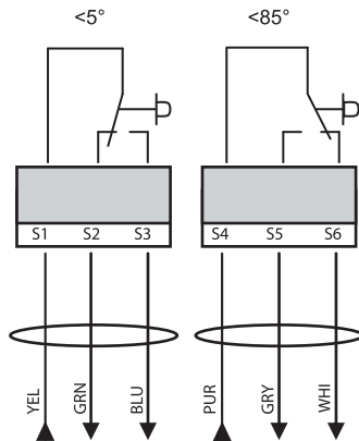
Auxiliary switches
