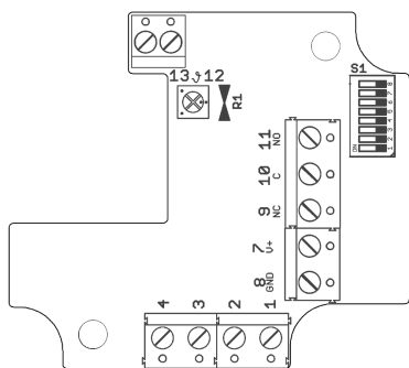
2-wire version
