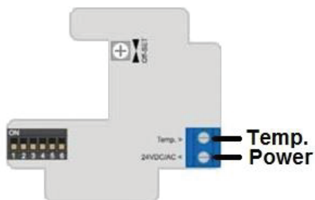
2-wire version
